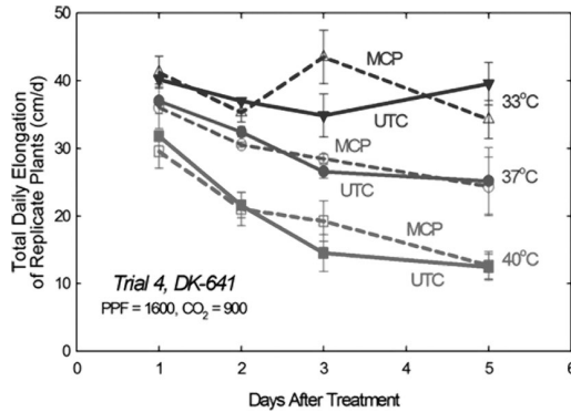
Figure 10. The effect of high temperature stress on leaf elongation of corn, with and without treatment of 1-MCP to block ethylene perception. 1-MCP did not result in a significant increase in leaf elongation at any of the three temperatures.
